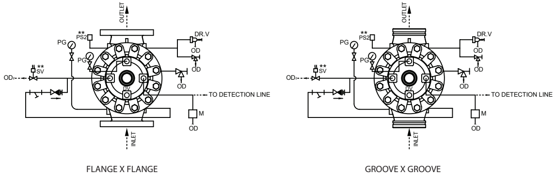
SCHEMATIC 5
