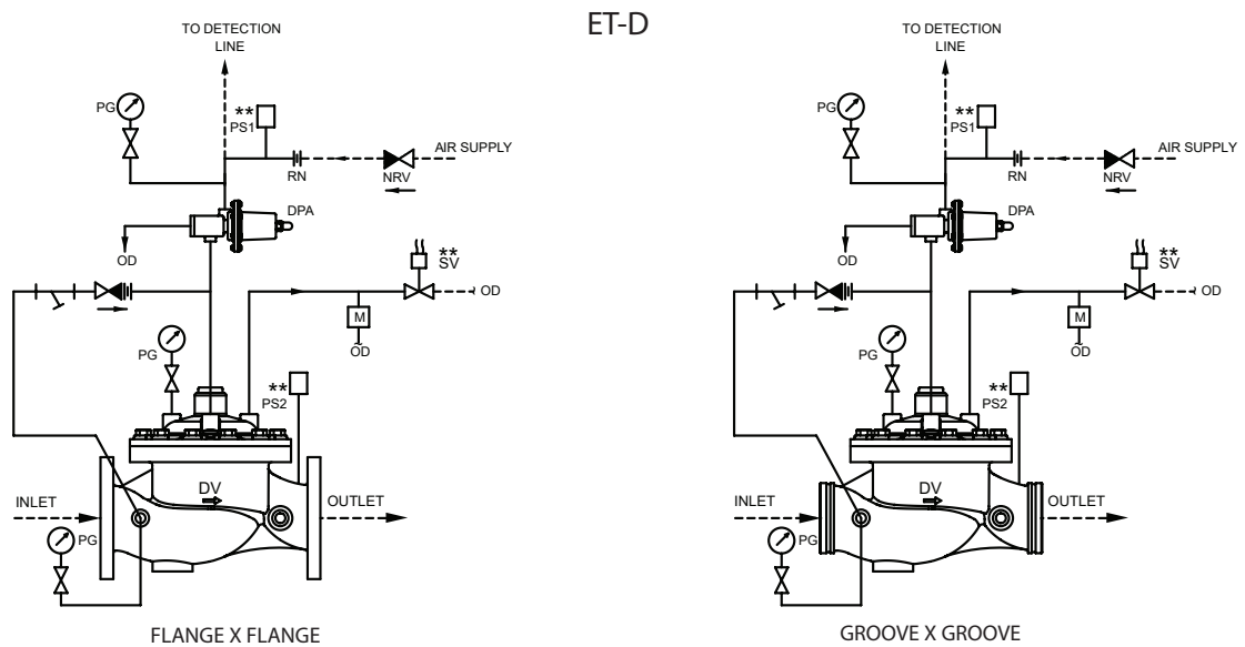
SCHEMATIC 10
