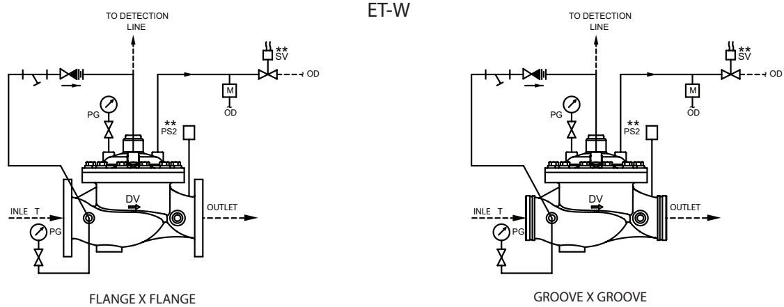
SCHEMATIC 9
