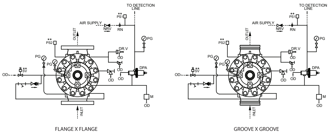
SCHEMATIC 6
