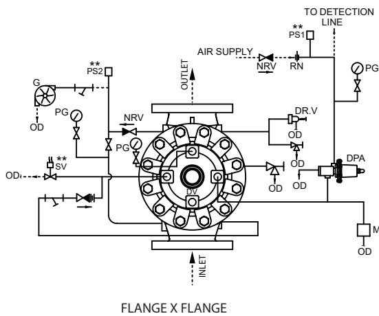
SCHEMATIC 8
