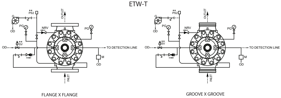
SCHEMATIC 3
