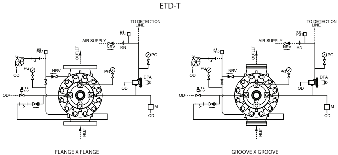
SCHEMATIC 4
