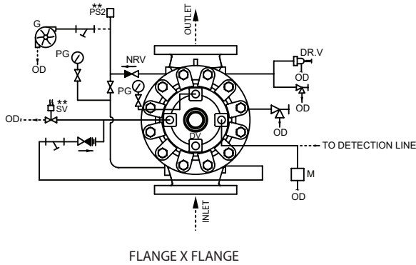
SCHEMATIC 7
